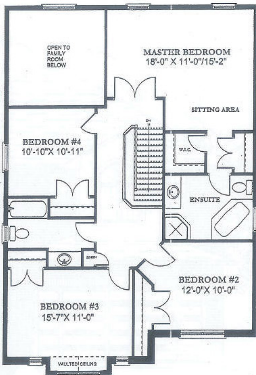
Second Floor - 1373 sf (including 157 SF of open area)
