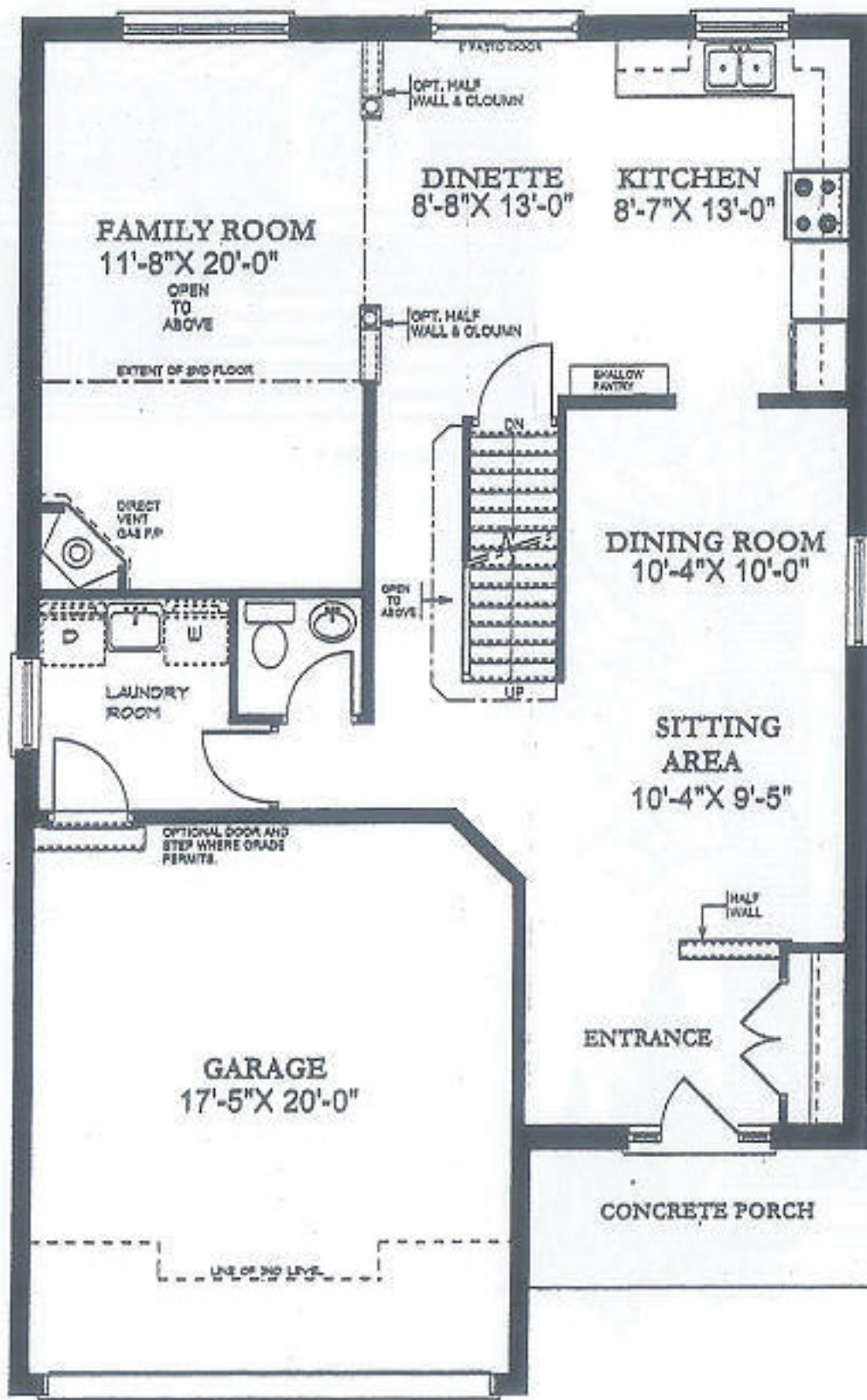
Ground Floor - 1072 sf
