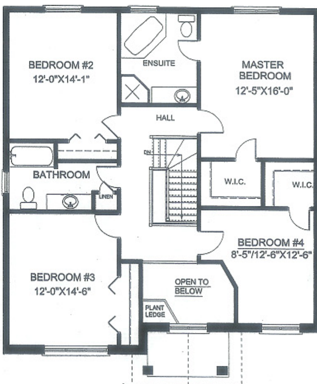
SECOND FLOOR PLAN 1152sf + 72sf of open area
