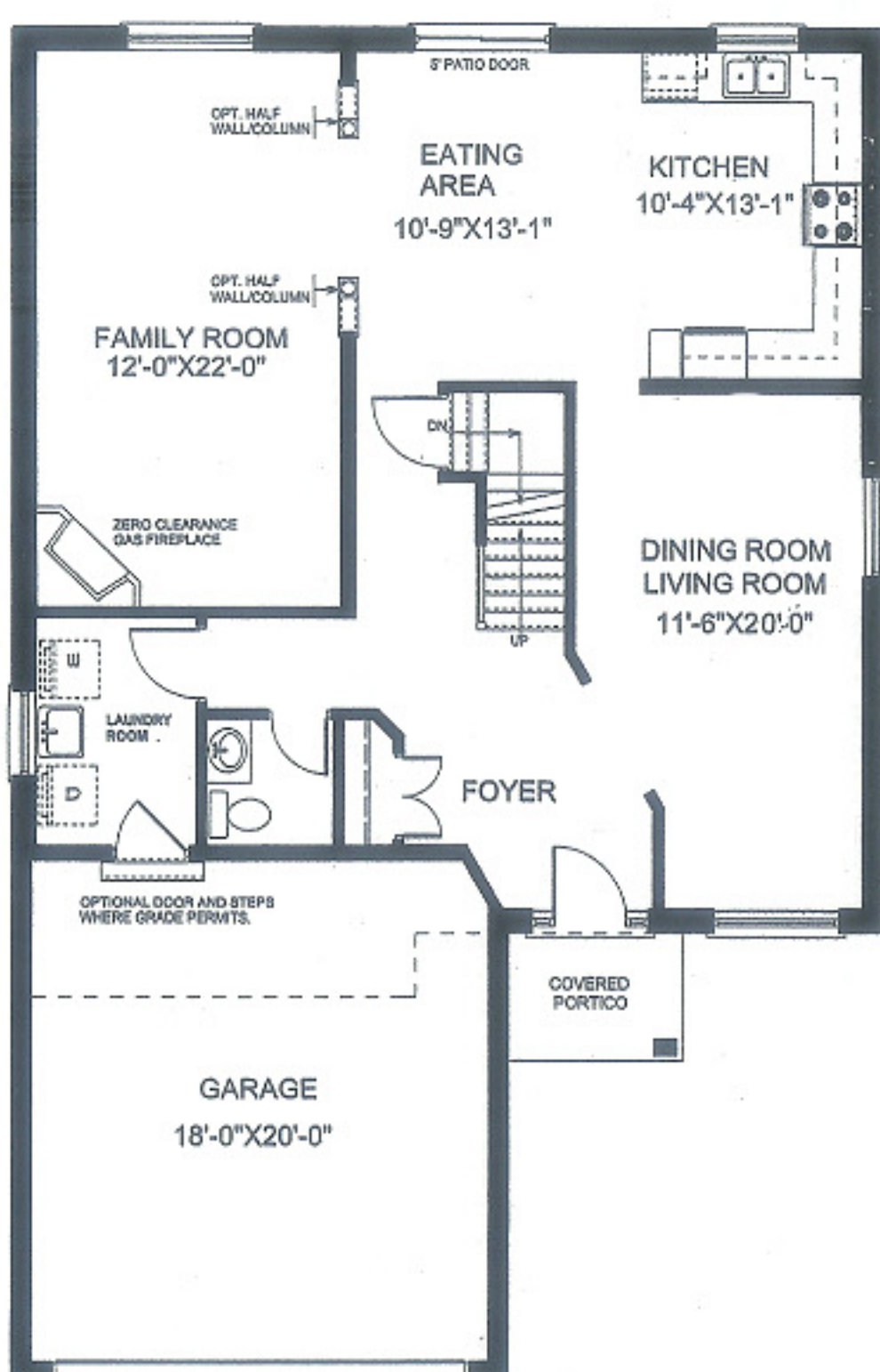
GROUND FLOOR PLAN 1164sf
