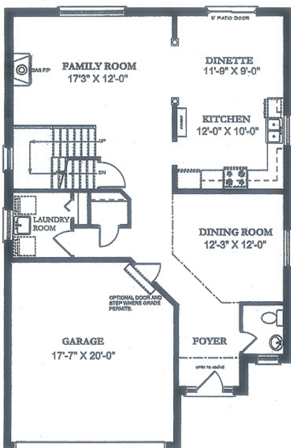
Ground Floor Plan 1056 SF
