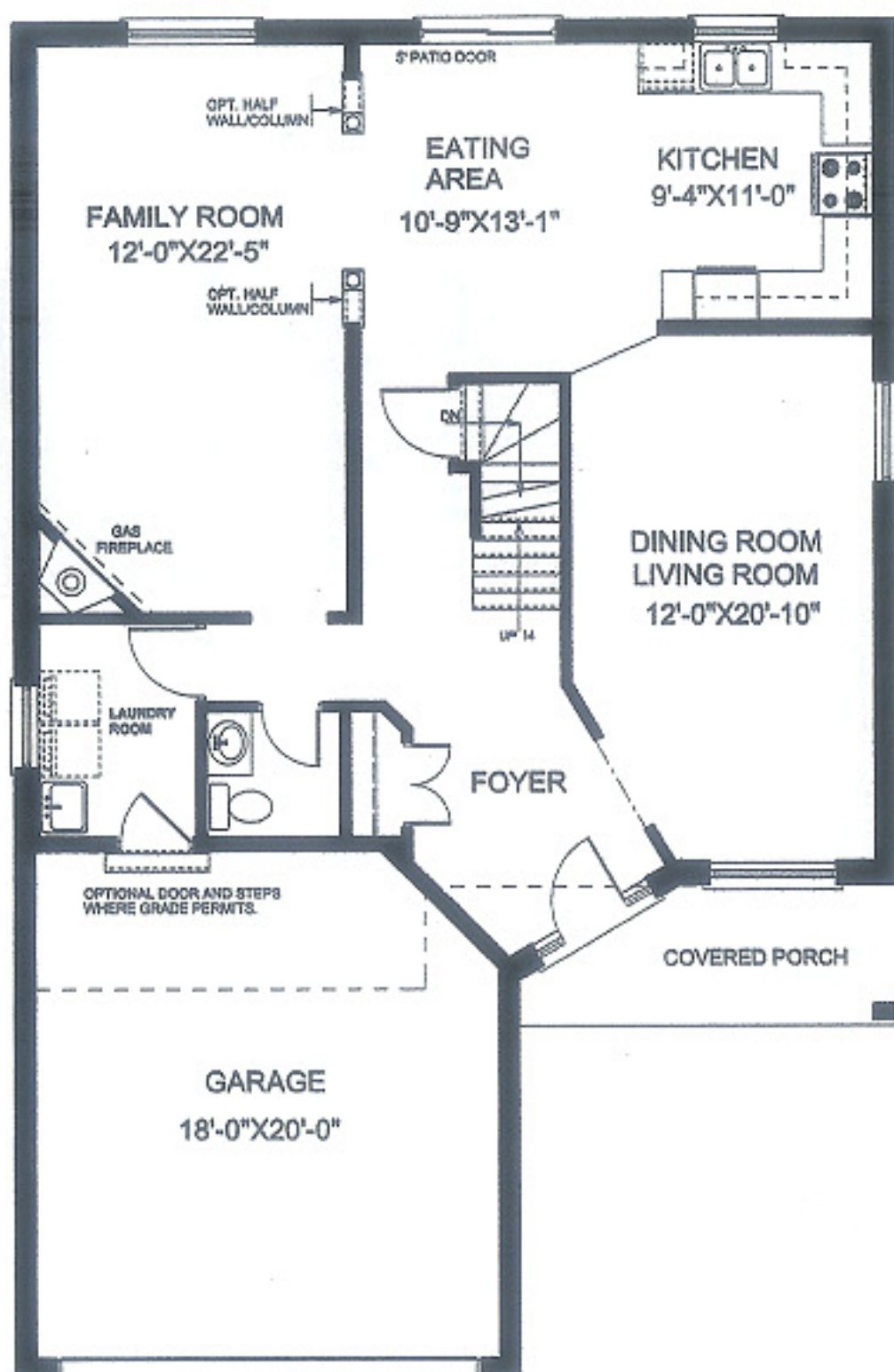
GROUND FLOOR PLAN 1167sf
