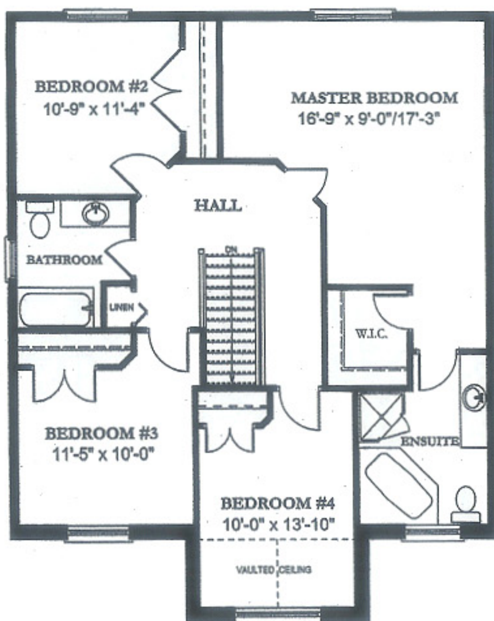
Second Floor Plan - 1103 sf
