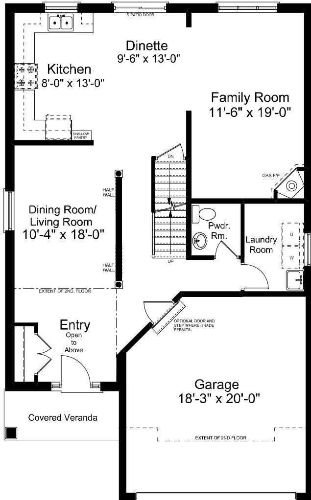
Ground Floor 1,058 sf
