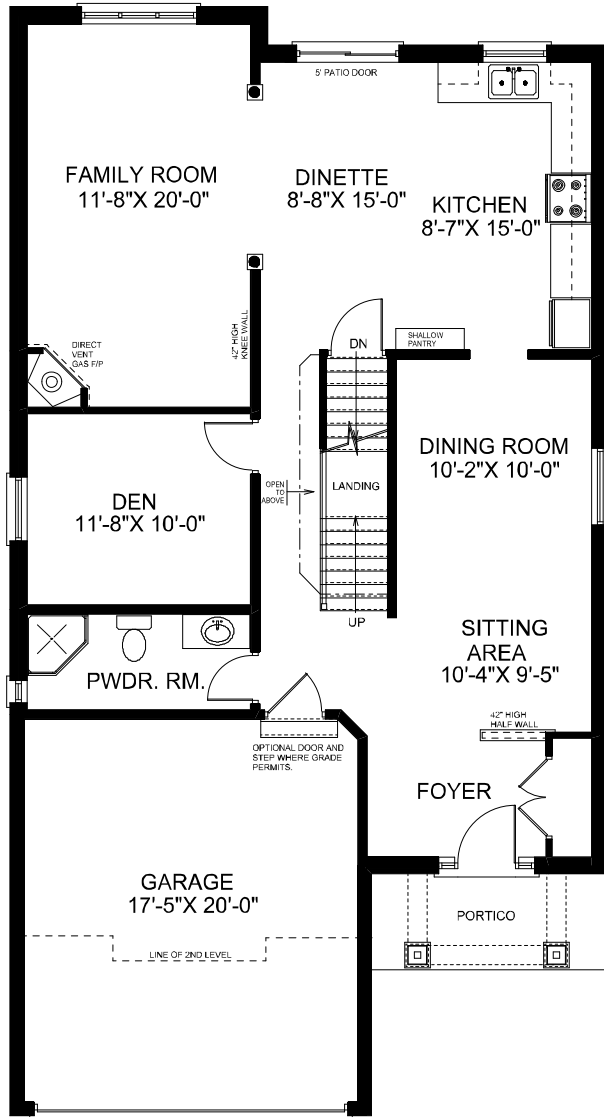
Ground Floor - 1222 sf
