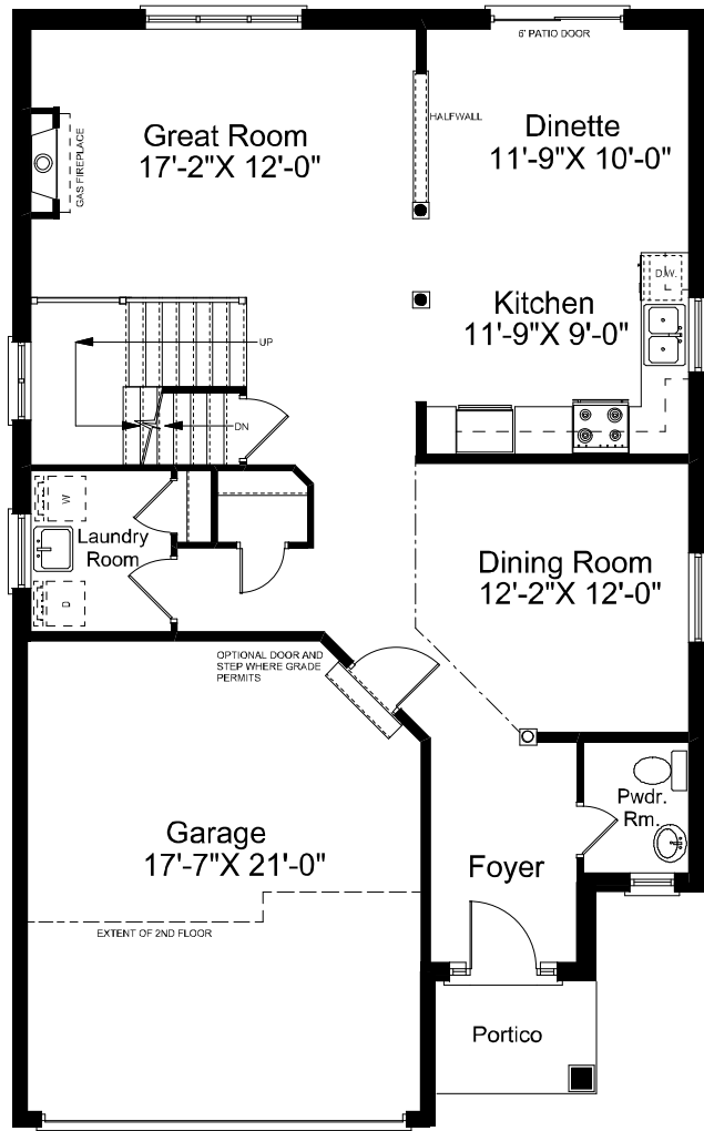
Ground Floor - 1068 SF
