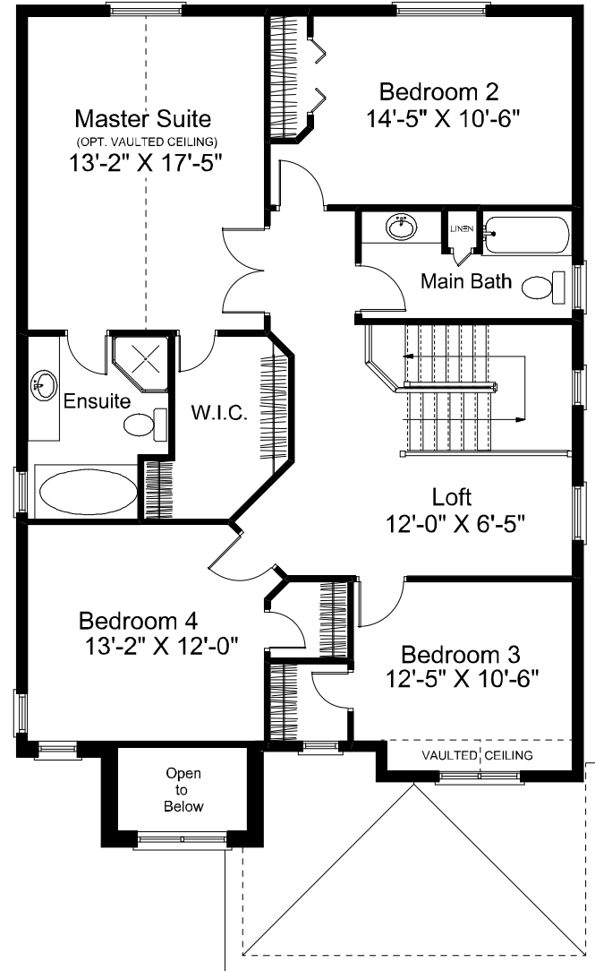
Second Floor Plan 1367 sf (incl. 38 sf of Open Area)
