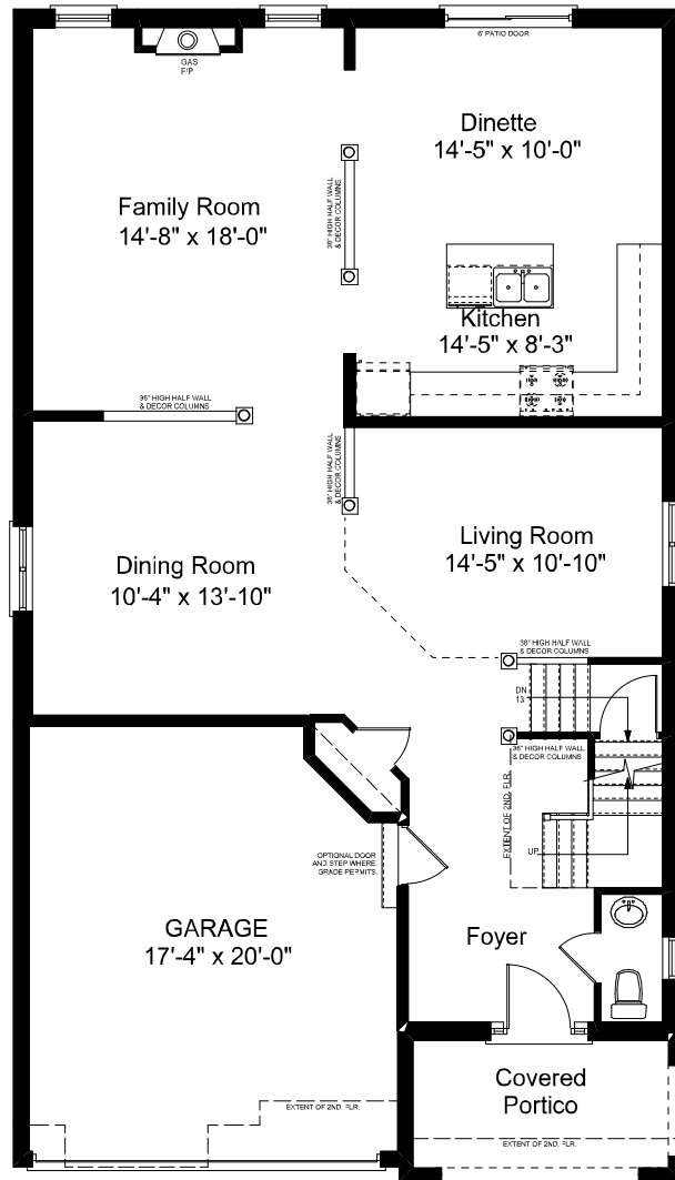
GROUND FLOOR - 1260sf
