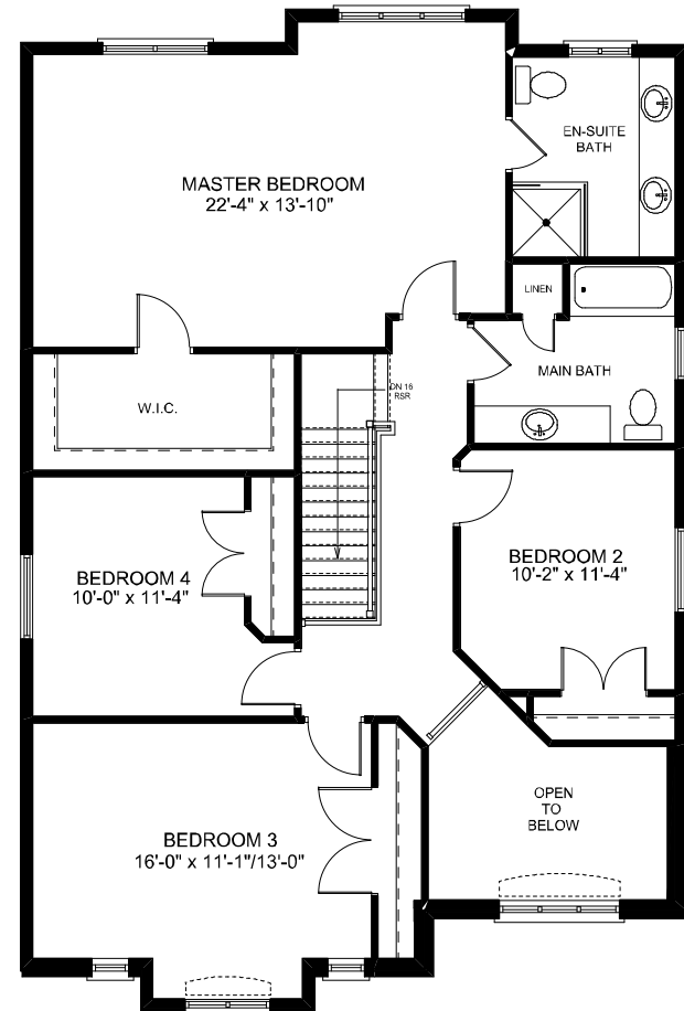
SECOND FLOOR- ELEVATION A 1386sf (including 95sf of open area)
