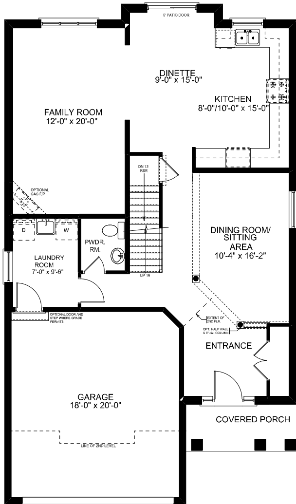
GROUND FLOOR 1125 SF
