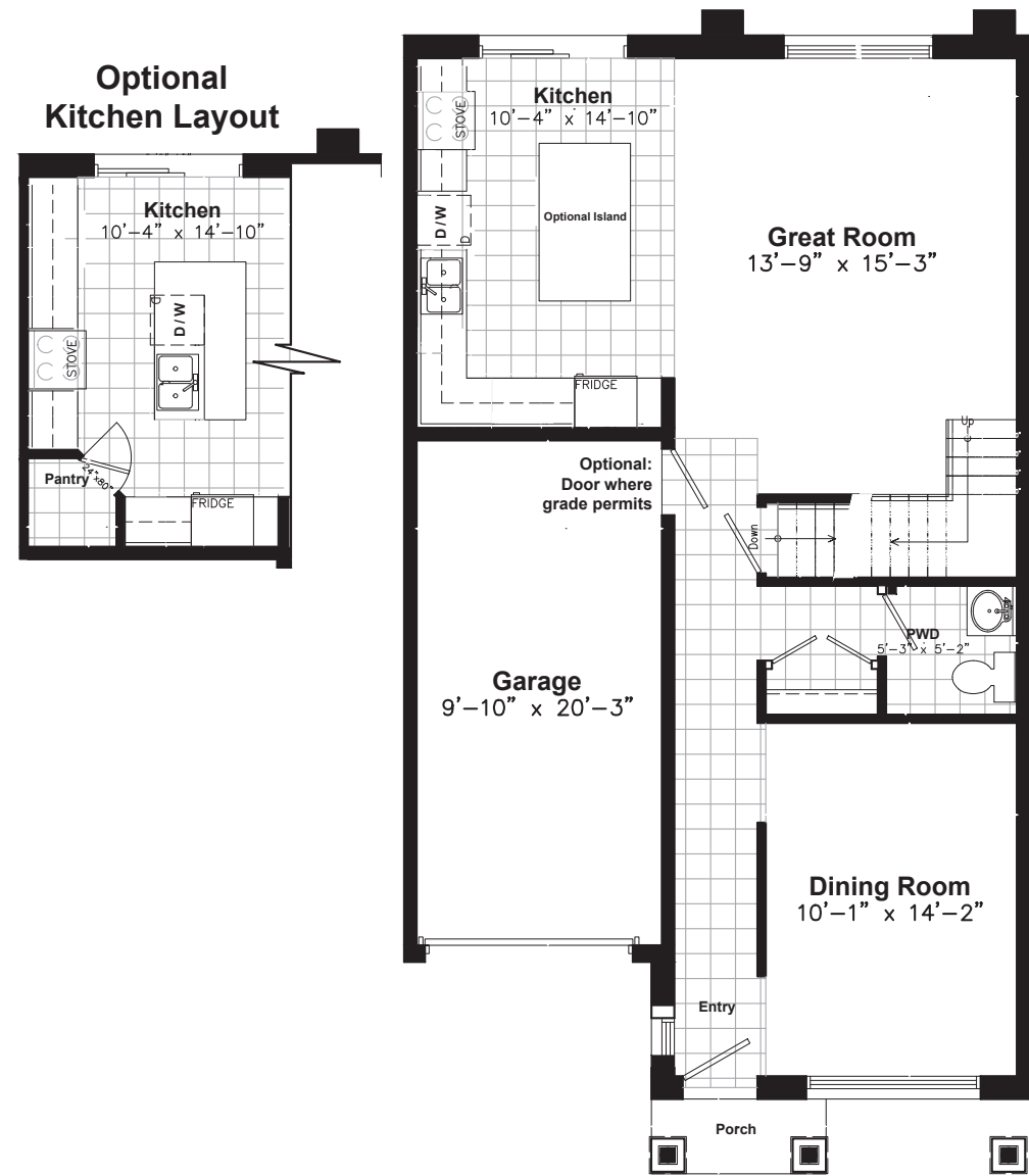
UNIT A FIRST FLOOR
